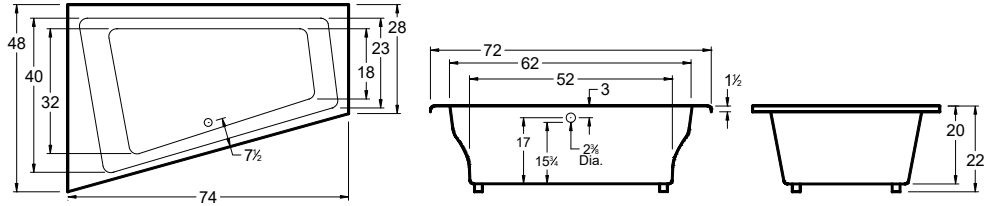
All bathtub dimensions are ± 1/2"
